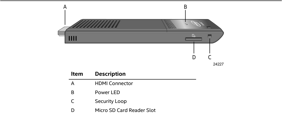
Figure 1. Left-Side View of Intel Compute Stick
